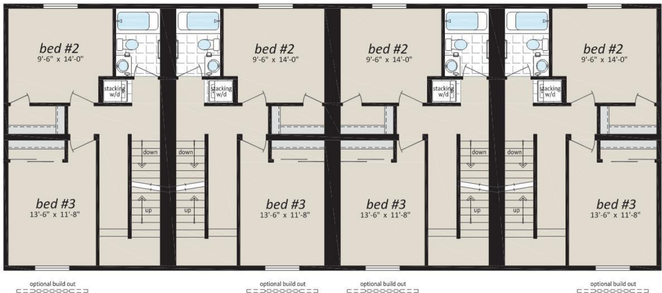
2nd Floor (Note: 3rd floor on next page)
